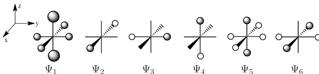
FIGURE 14.2 – Orbitales du fragment L_6
